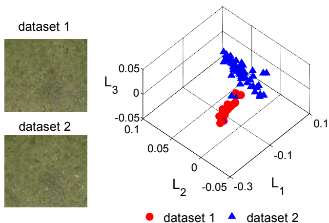
Figure 2: Change in process conditions is detected by an online computer vision system by projection of froth image features to a control chart.
