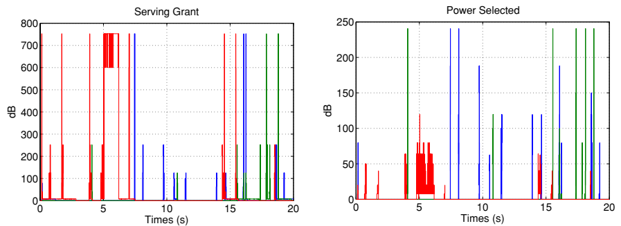
Simulation of allocated grants (serving grants) and used grants (selected power)
