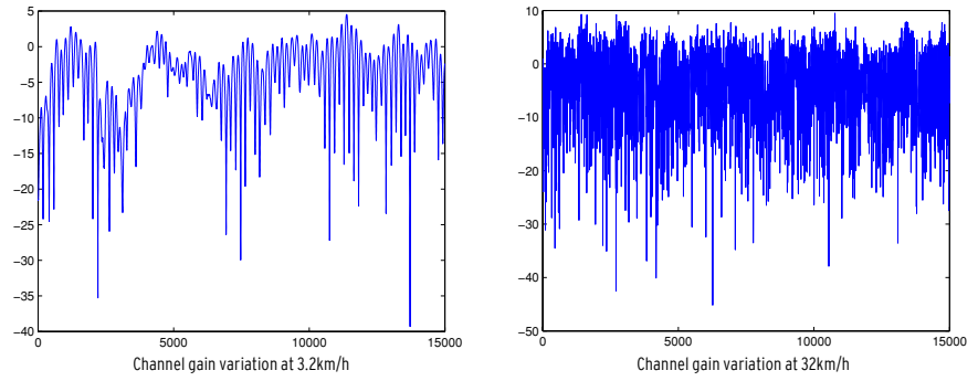
Illustration of fading at different user speeds
