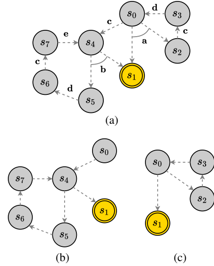
Figure 2: Minimal Critical-Value example.
