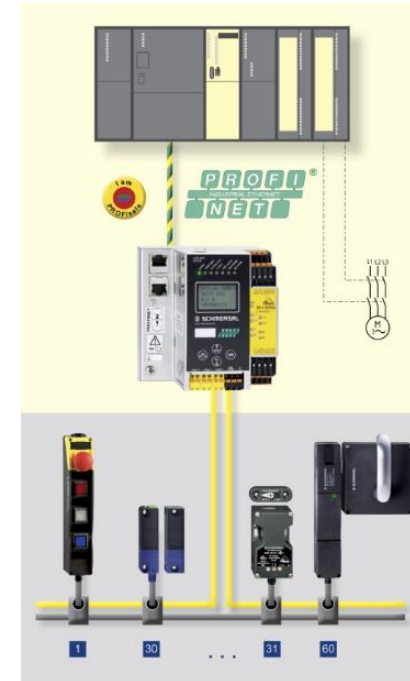
Safety gateways ("Safety integrated")
