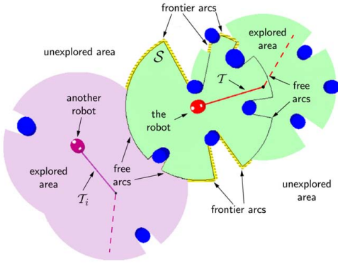
Fig. 4. Frontier, free and obstacle arcs in the Local Safe Region S .
