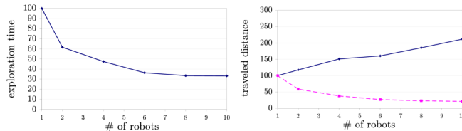
Fig. 12. Garden exploration with clustered start: exploration time (left) and total traveled distance (right, solid blue line) with teams of different cardinality for limited communication range. Also shown is the average distance traveled by each robot (right, dashed violet line).
