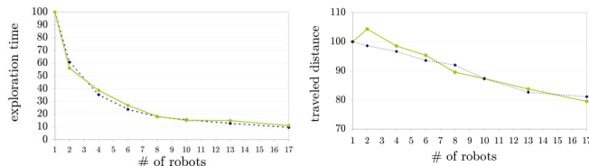
Fig. 9. Garden exploration with scattered start: exploration time and total traveled distance with teams of different cardinality for unlimited (dotted line, blue) and limited (solid line, green) communication range.
