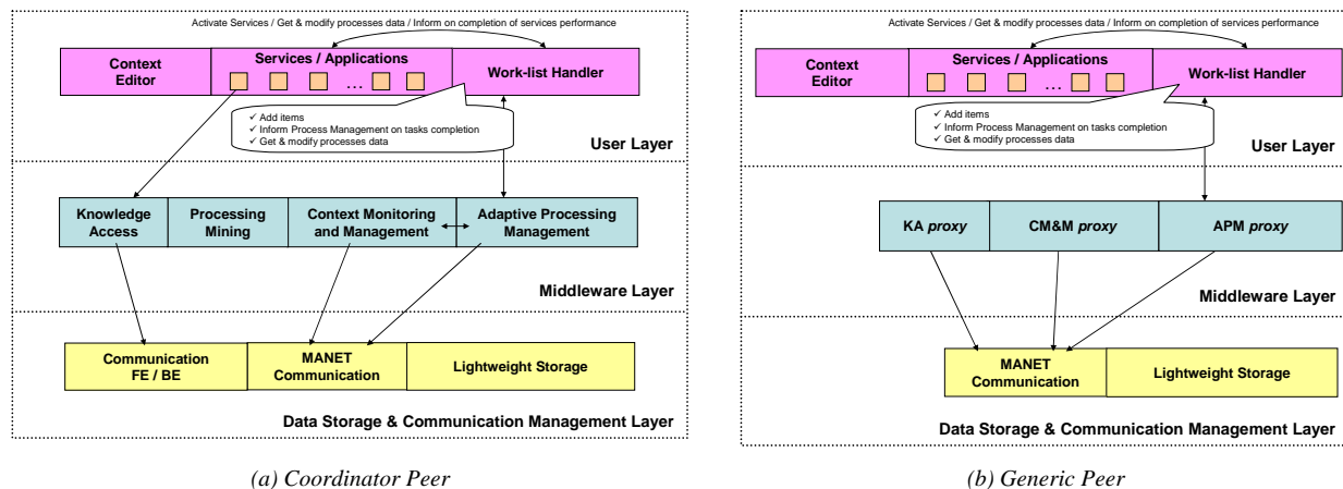
Figure 4. Front-end Architecture
