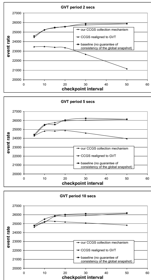
Figure 5. Execution Speed Results.
