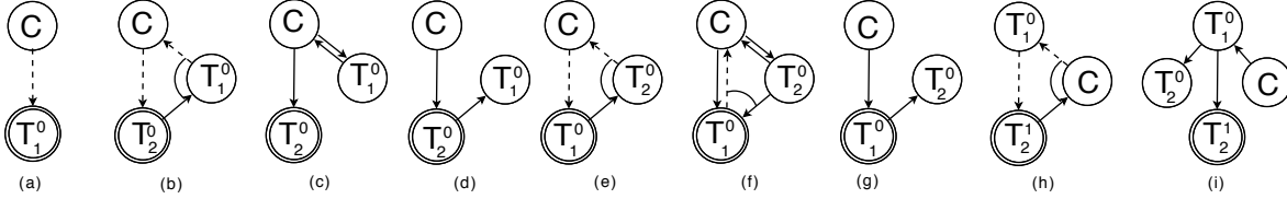
Fig. 6. SCC Execution for History \mathcal{H}_3
