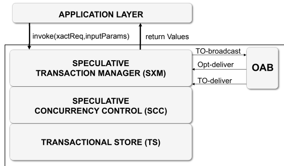
Fig. 1. Software Architecture of Each Process
