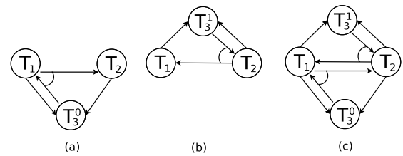
Fig. 3. Polygraphs Associated with Histories \mathcal{H}_1 and \mathcal{H}_2
