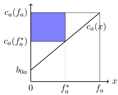
Figure 4: Illustration of the proof of Theorem 4.4
