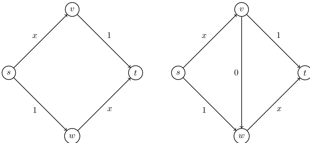
Figure 3: Braess' paradox
