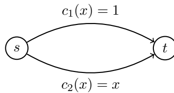
Figure 1: Pigou's network
