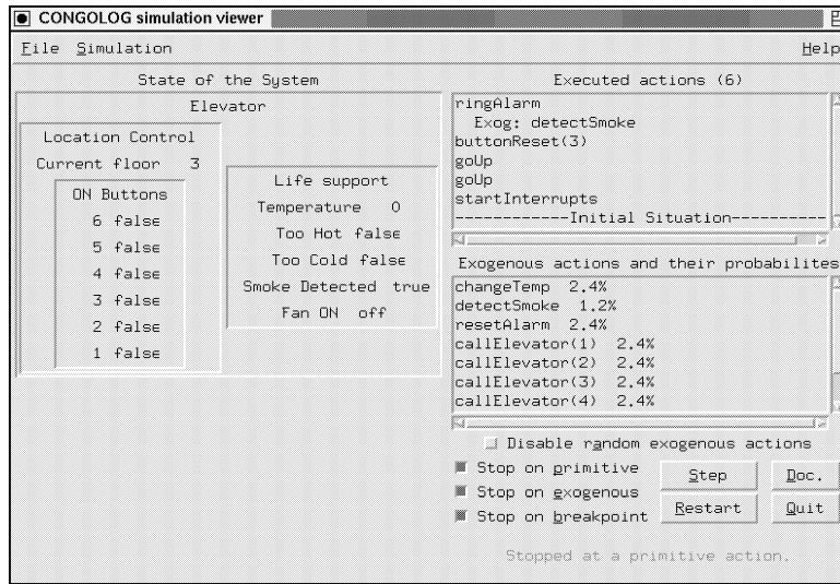
Fig. 1. The ConGolog toolkit's graphical viewer.
