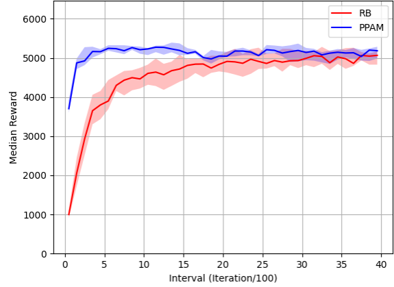
Figure 2: Median reward of PPAM and RB agents.
