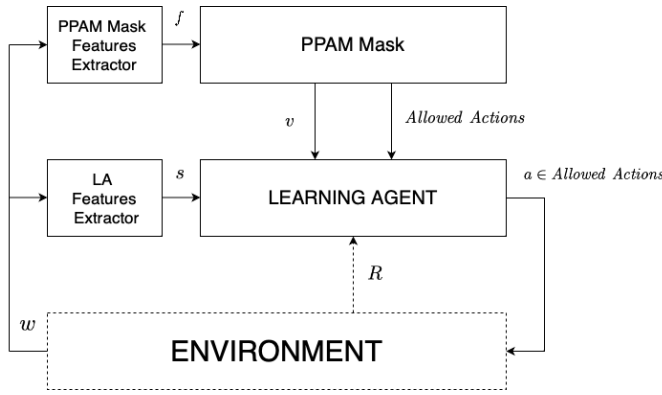
Figure 1: Interaction between the environment, agent and the PPAM mask. Allowed\ Actions \subseteq A(s) is the set of permitted actions output by the PPAM mask, v \in \mathcal{L} is the PPAM mask’s state, a \in Allowed\ Actions is the action chosen by the agent, R is the reward given by the environment after a is performed, and w is the resulting state of the environment. From w , we obtain the MDP state s through the learning agent’s feature extractor, and f through the feature extractor of the PPAM mask (notice these need not be aligned).
