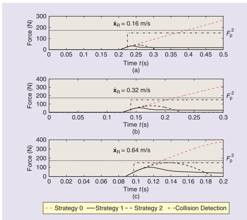
Figure 4. Stabbing simulation with the full dynamic model of the LWR-III equipped with a knife. The fully covered human stands 0.3 \text{ m} before the stretched out singularity of the robot. F_p^2 denotes the penetration force for the fully covered skin.
