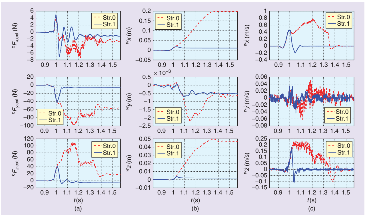
Figure 11. Time evolution of cutting with and without collision detection. (a) Contact force, (b) position, and (c) velocity.
