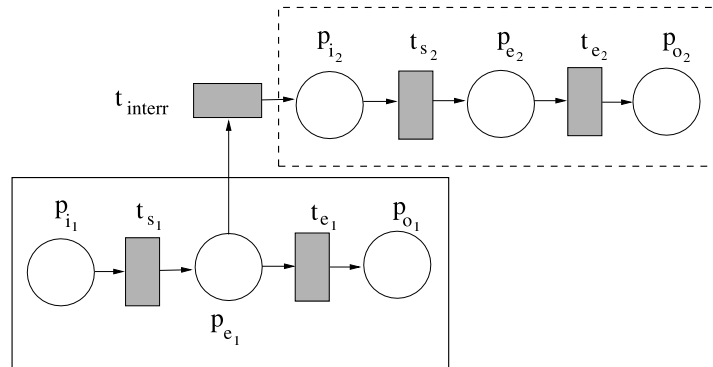
Fig. 9. Interrupt structure where possibly T_1 is interrupted and then T_2 executed.
