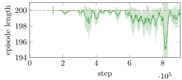
Figure 6: Dueling DQN algorithm with and without our RS. Training episode lengths, averaged over 5 runs.
