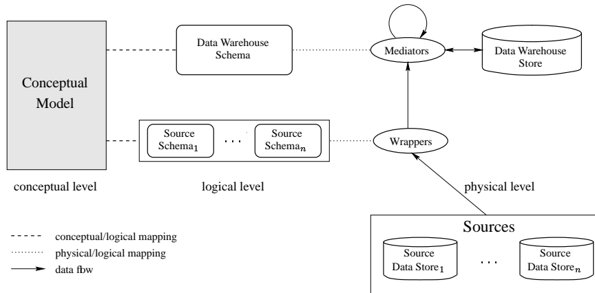
Figure 1. Architecture for Data Integration
