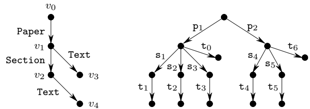
Figure 1: Schema for papers divided in sections and a conforming database
