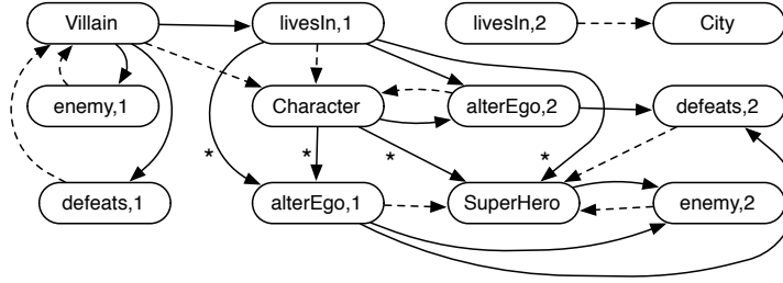
Figure 3: Weakly acyclic dependency graph for Example 1.
