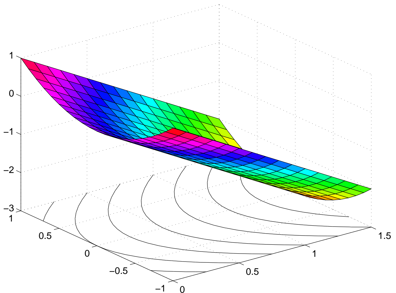
Figure 3.7: Plot of q(x_1, x_2) when \alpha = 0 \beta = 1 .
