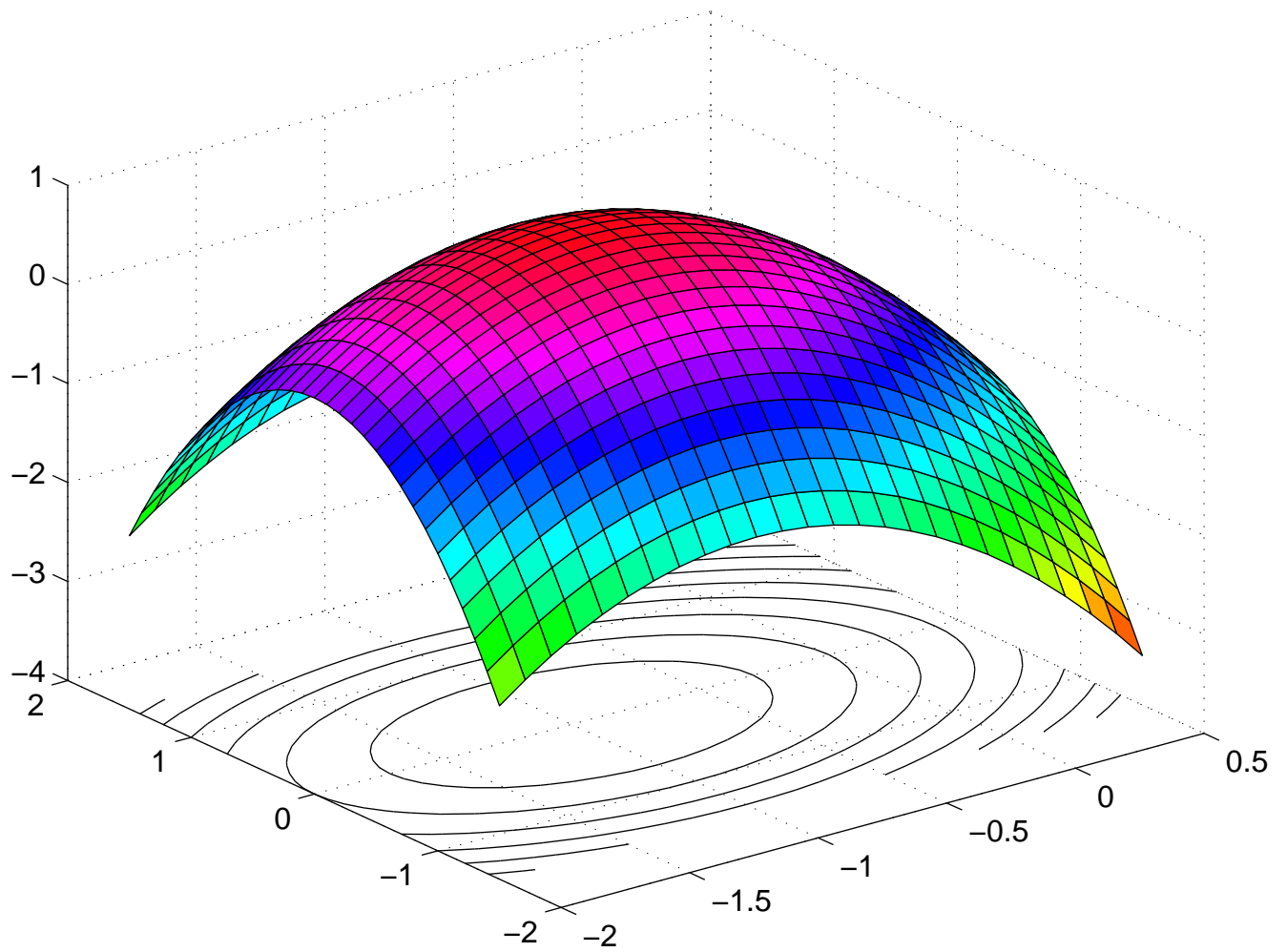
Figure 3.10: Plot of q(x_1, x_2) when \alpha = \beta = -1 .
