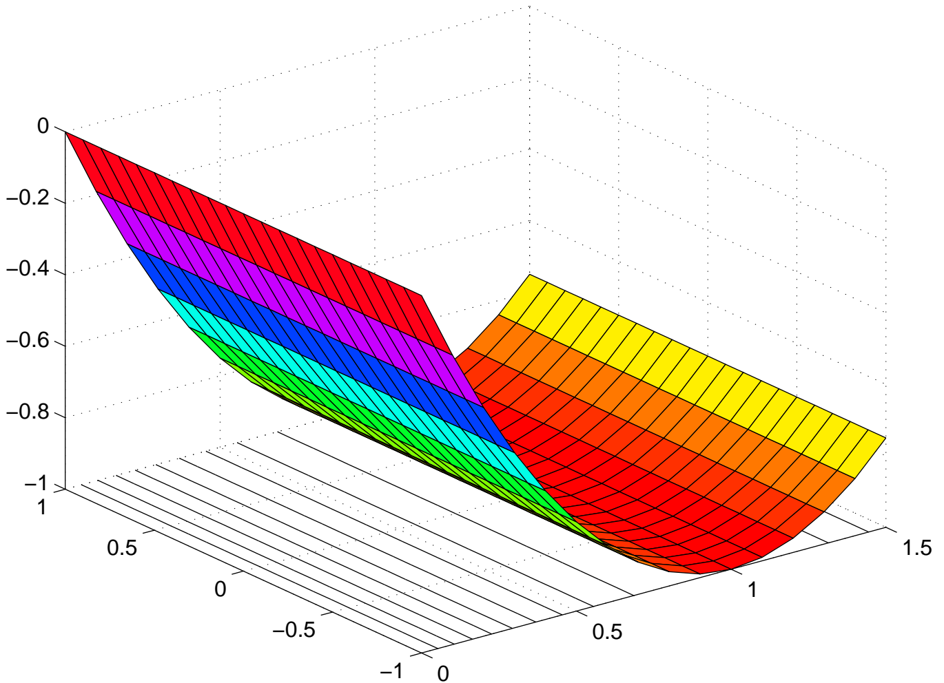
Figure 3.8: Plot of q(x_1, x_2) when \alpha = 1 \beta = 0 .
